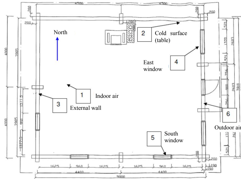
Fig. 2. Location of dataloggers in case building 5.
