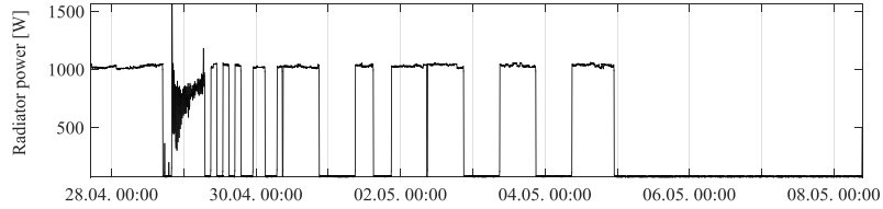
Fig. 3. Power supplied to the radiator during Experiment 6
