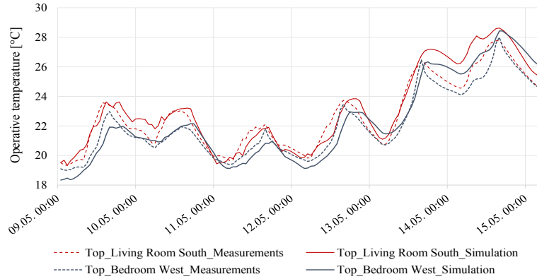
Fig. 5. Operative temperature trend in the Living Room South and the Bedroom West during Experiment 7
