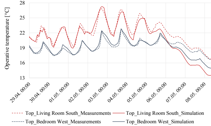
Fig. 4. Operative temperature trend in the Living Room South and Bedroom West at the end of the calibration
